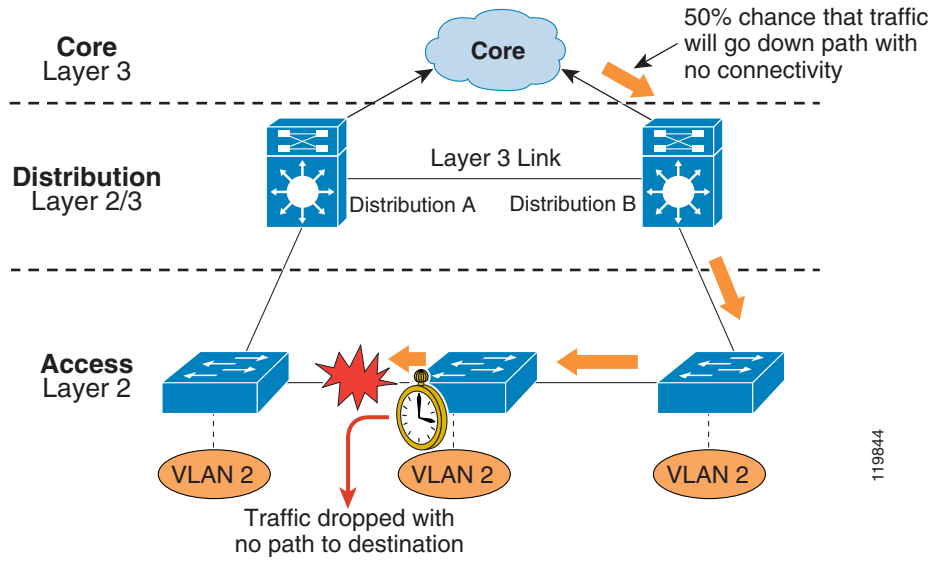
Figure 47 Dropped Traffic
