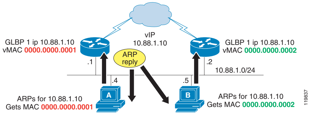
Figure 38 GLBP Operation
