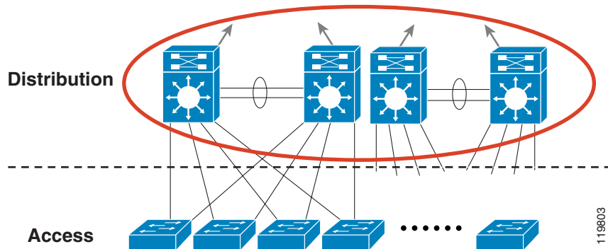
Figure 3 Distribution Layer
