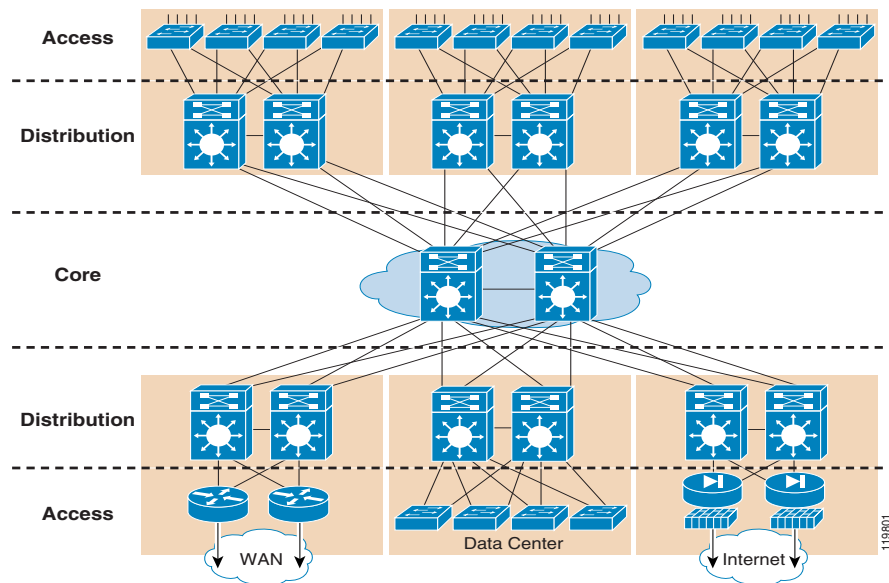
Figure 4 Distribution Layer—High Availability
