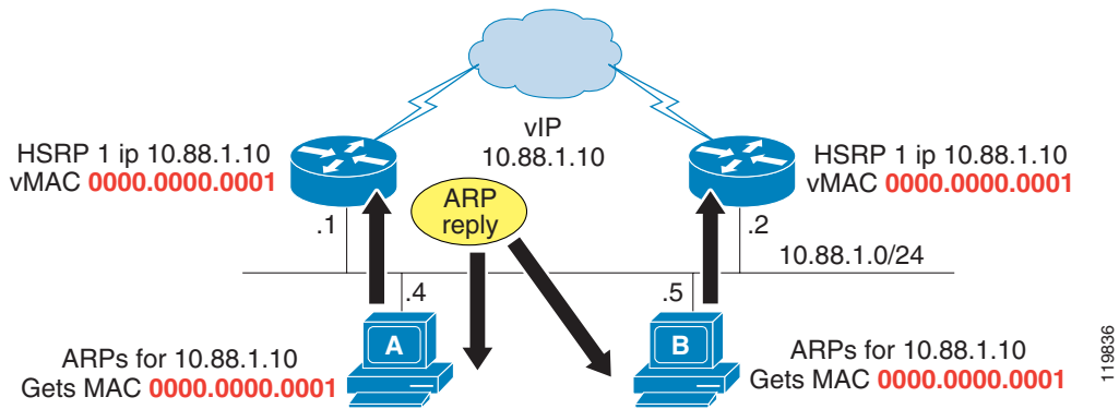
Figure 37 HSRP Operation
