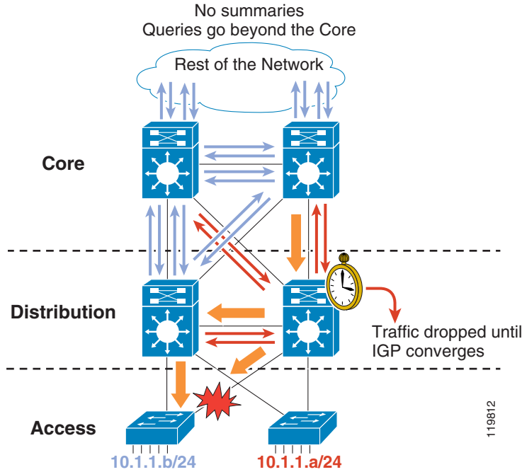
Figure 13 Convergence Around a Failed Node
