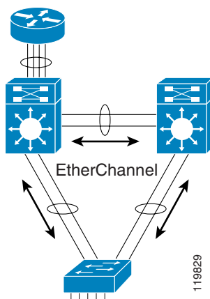
Figure 30 EtherChannels
