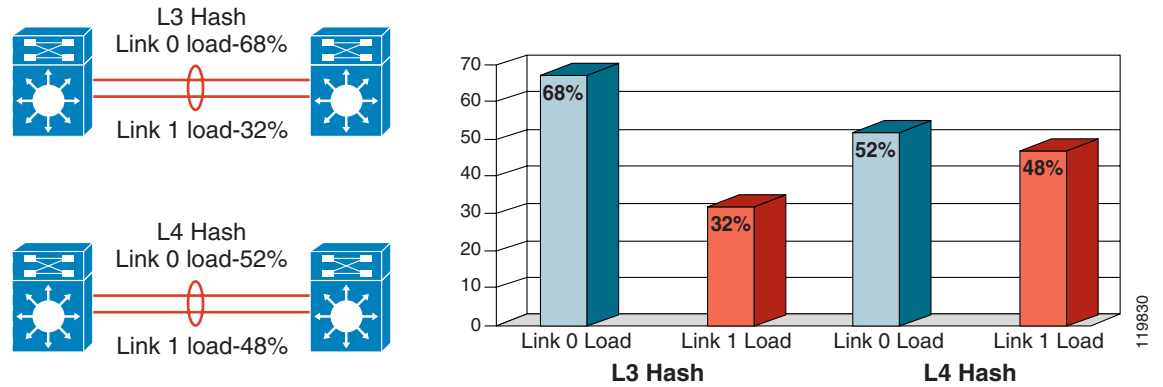
Figure 31 EtherChannel Testing Results
