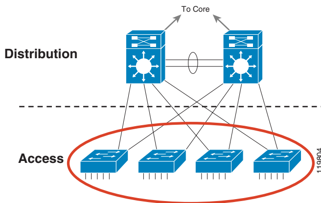
Figure 5 Access Layer
